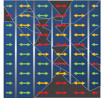
Figure 5: Not only are the smaller cells of the Performance panel less susceptible to breakage, but they confine cracks to a smaller portion of the panel, while maximising energy generation through a series of redundant electrical connections.
